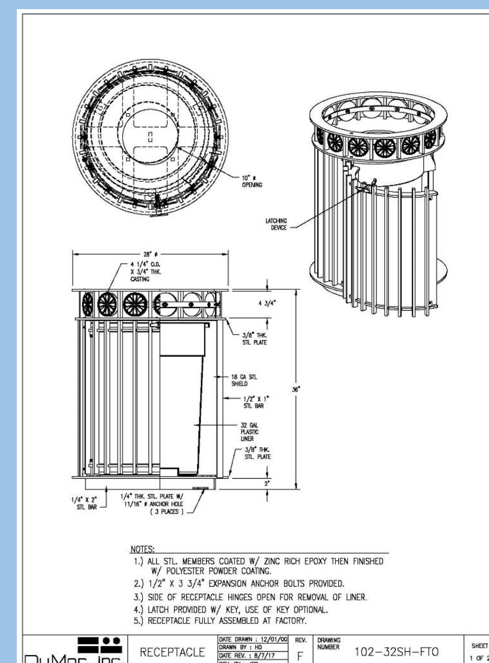
Trash Receptacle
