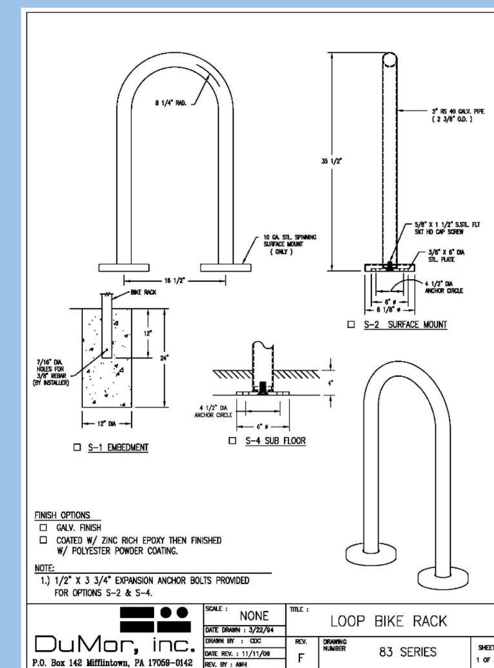
Bicycle Rack
