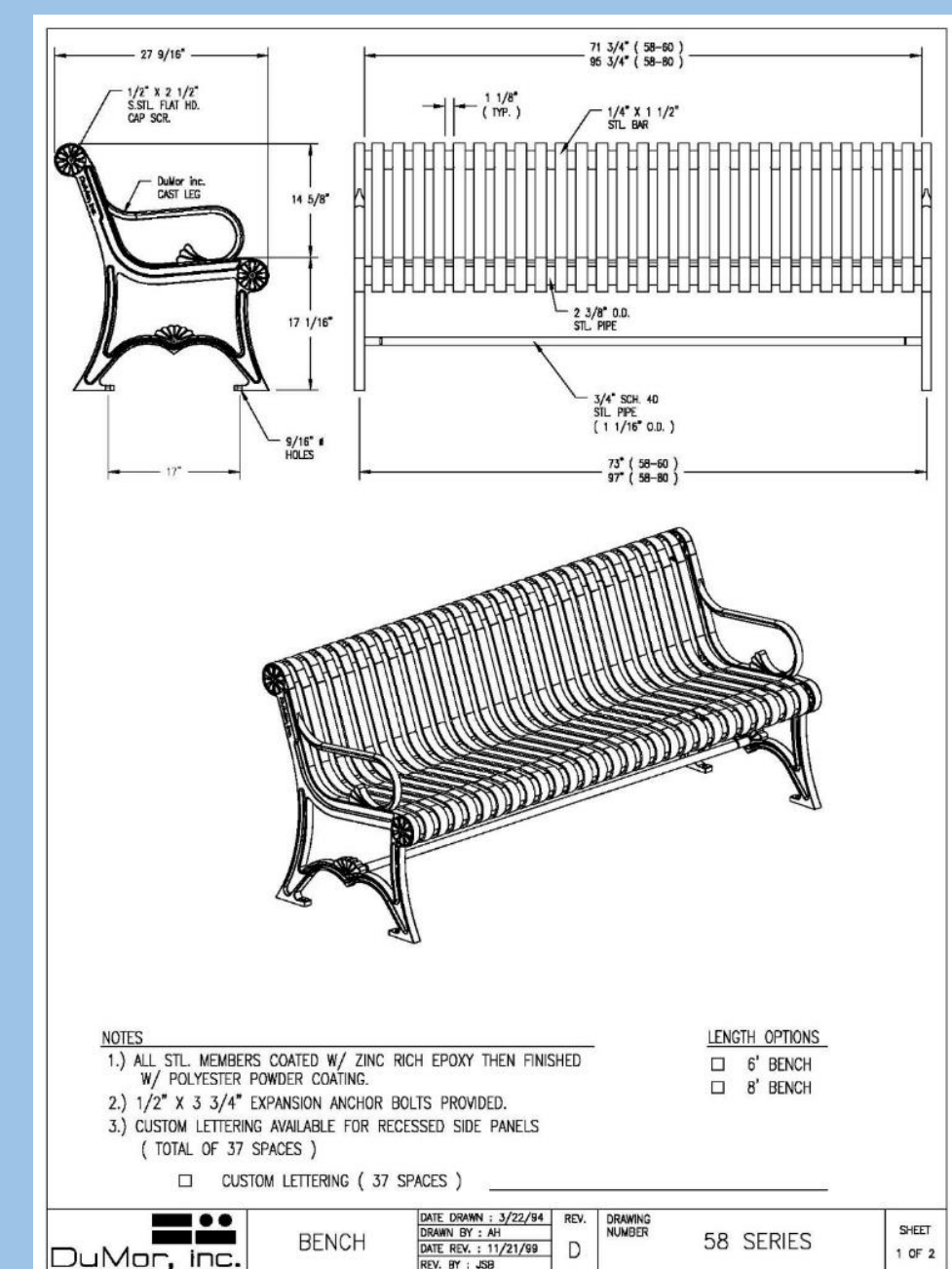
Bench
